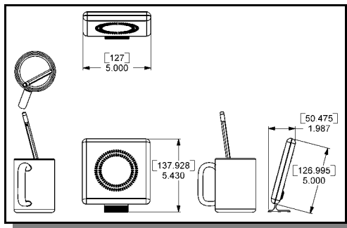
Figure 10—Physical Dimensions
